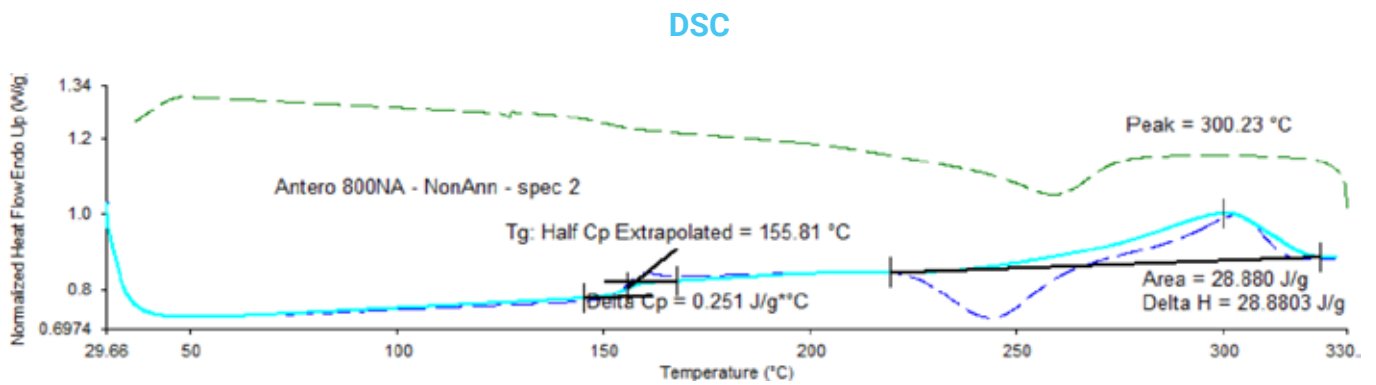
Figure 1: 2nd Heating Scan, DSC, for Antero 800NA
